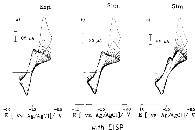
Figure 15. Experimental and simulated cyclic voltammograms of 35 . Simulation data: C^* = 8 \times 10^{-4} M, E_{A_1}^{\circ} = -1.66 V, E_{B_2}^{\circ} = -1.49 V, k_{s(A_1)} = 1.7 \times 10^{-3} cm s ^{-1} ( \alpha = 0.55 ), k_{s(B_2)} = 2.6 \times 10^{-3} cm s ^{-1} ( \alpha = 0.52 ), D = 2.1 \times 10^{-6} cm ^2 s ^{-1} , k_{AB} = 180 s ^{-1} , k_{BA} = 20 M ^{-1} s ^{-1} , electrode area = 7.9 \times 10^{-3} cm ^2 , v = 400 mV s ^{-1} , E_{A_1} = -1.85 V, E_{A_2} = -1.25 V. (a) Experiment (see Figure 13); (b) ECE/EEC disproportionation mechanism, disproportionation reaction in dynamic equilibrium; (c) ECE/EEC mechanism.
