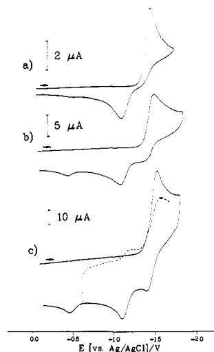
Figure 11. Cyclic voltammograms of 9.2 \times 10^{-4} M 21 in \text{CH}_3\text{CN}/0.1 M \text{TBAPF}_6 , T = 24 °C. (a) v = 0.4 \text{V s}^{-1} ; (b) v = 50 \text{V s}^{-1} ; (c) v = 150 \text{V s}^{-1} ; dashed line, second forward sweep ( E_\lambda = -0.7 V).
