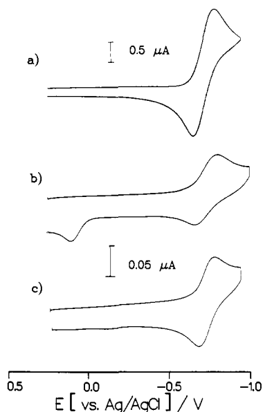
Figure 2. Cyclic voltammograms of 1 in dry acetonitrile with 0.1 M \text{TBAPF}_6 as supporting electrolyte; scan rate 0.2 \text{ V s}^{-1} ; T = 24^\circ \text{C} . (a) 2.4 \times 10^{-3} \text{ M} ; (b) 7.2 \times 10^{-5} \text{ M} ; (c) 7.2 \times 10^{-5} \text{ M} after addition of CO.
