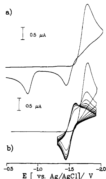
Figure 13. Cyclic voltammograms of 8.0 \times 10^{-4} M 35 in \text{CH}_3\text{CN}/0.1 M \text{TBAPF}_6 , scan rate: 0.4 \text{ V s}^{-1} , T = 24 °C. (a) Single sweep cyclic voltammogram; (b) multisweep cyclic voltammogram scanned between -1.25 and -1.85 V.
