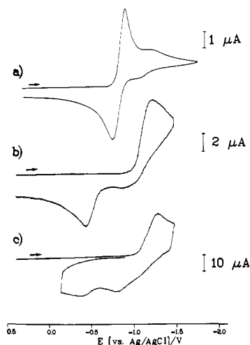
Figure 9. Cyclic voltammograms of 9.4 \times 10^{-4} M 14 in \text{CH}_3\text{CN}/0.1 M TBAPF 6 . (a) v = 0.3 V s -1 , T = 24 °C; (b) v = 10 V s -1 , T = -43 °C; (c) v = 150 V s -1 , T = -43 °C.
