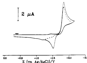
Figure 14. Cyclic voltammogram of 8.0 \times 10^{-4} \text{ M} 35 in the presence of a 35-fold excess of \text{PEt}_2\text{Ph} . T = 24 \text{ }^\circ\text{C} . Scan rate: 0.4 \text{ V s}^{-1} . Dashed line: second forward sweep ( E_{\text{A}} = -1.25 \text{ V} ).
