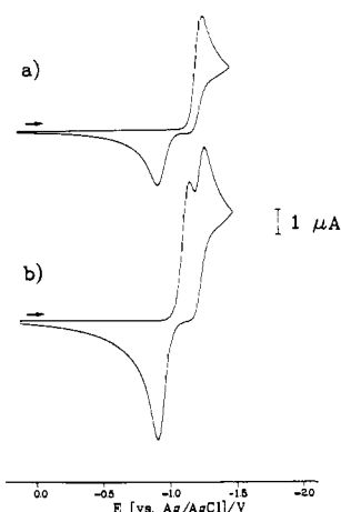
Figure 10. Comparison of the reduction products of 12 and 14 by cyclic voltammetry: scan rate = 0.2 V s -1 , T = -10 °C, \text{CH}_2\text{Cl}_2/0.1 M TBAPF 6 . (a) 1.6 \times 10^{-3} M 12 ; (b) 1.6 \times 10^{-3} M 12 + 1.5 \times 10^{-3} M 14 .
