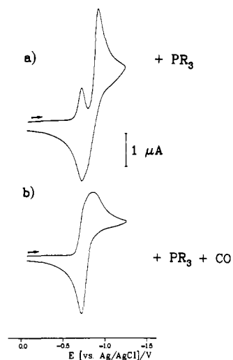
Figure 3. Cyclic voltammograms of 9.0 \times 10^{-4} \text{ M} 1 in \text{CH}_3\text{CN}/0.1 \text{ M TBAPF}_6 (a) in the presence of 3.1 mM \text{PPh}_3 and (b) after further addition of CO (saturated solution). Scan rate = 0.3 \text{ V s}^{-1} , T = 24^\circ \text{C} .
