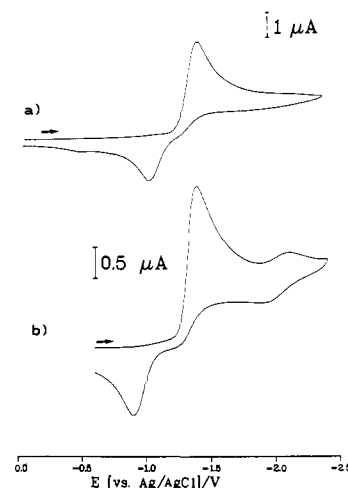
Figure 12. Cyclic voltammograms of 9.2 \times 10^{-4} M 21 in \text{CH}_3\text{CN}/0.1 M \text{TBAPF}_6 . Scan rate: 0.2 \text{V s}^{-1} . (a) T = 24 °C; (b) T = -10 °C.
